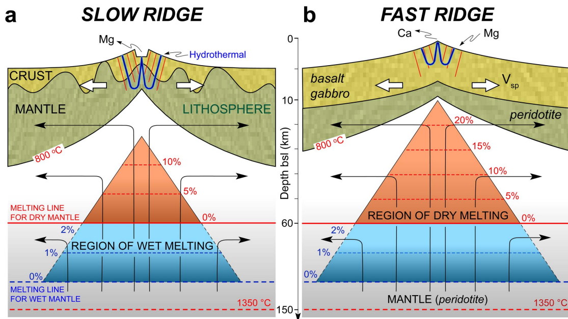
Figure 3 | Effects of spreading rate on the possibility of MORP-seawater reactions during hydrothermal circulation at mid ocean ridges. Assuming a constant mantle potential temperature of 1350 °C at a depth of 150 km and plate thickening passive flow, the degree of melting of the upwelling mantle depends on whether plate separation is slow (a) or fast (b). We solved for the steady-state three-dimensional passive mantle flow via a Fourier pseudo-spectral technique 44 . The base of rigid plates, assumed to correspond to the depth of the 800 °C isotherm, was obtained iteratively solving each time the mantle temperature field, starting from a constant-thickness plate-flow model. Streamlines show a schematic passive corner flow in the asthenosphere. The shaded triangles indicate the fraction of melt generated across axis, including the effect of water on peridotite solidus. Assuming a ~ 0.02 wt% H 2 O content in the upper mantle, the peridotite solidus is lowered causing partial melting in a subridge mantle region wider and deeper than if the mantle were dry. The faster the mantle rises, the shallower melting ends. As a result, more mantle melts, creating a thicker basaltic crust and shallow seawater penetration, with little chance for mantle ultramafics to interact with seawater and to release Mg to the ocean. Slow ridge MORP-seawater reactions may result in Mg release to the ocean.
