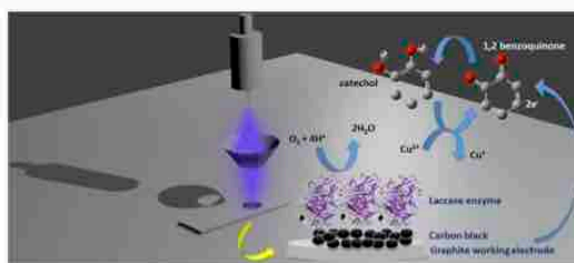
Figure 1: Schematic of ESI apparatus for deposition at ambient pressure and laccase catalysed red-ox reaction of catechol pollutant.
