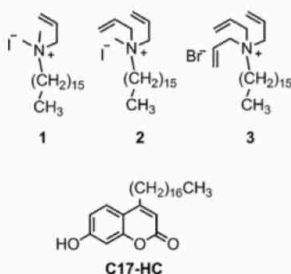
Chart 1. Fluorescent probe C17-HC and cationic amphiphiles 1–3
