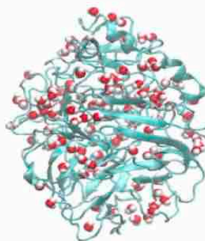
Figure 1B Laccase structure after 300 ns
