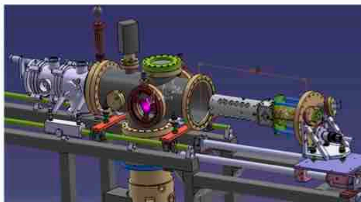
Figure 1. The electro-spray ionization (ESI) source, in-vacuum transfer and mass/charge selection.
