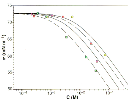
Surface tension lowering by organics in cloud water. Surface tension decrease with respect to pure water as a result of water-soluble organic carbon in cloud water (expressed as moles per liter of carbon). Data from Tenerife (Spain) and Po Valley (Italy) taken by one of the authors (M.C.F.).
