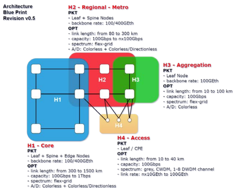
Figura 4: GARR-T Blue Print Architecture
