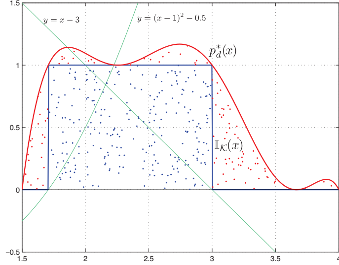
Fig. 8. Illustration of the behavior of Algorithm 1 in the one-dimensional case. Blue dots are accepted samples, red dots are rejected samples.
