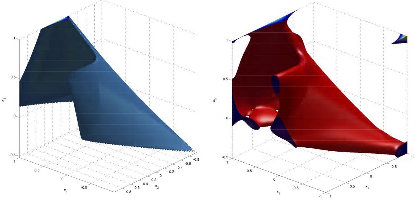
Fig. 5. Left: set of stabilizing PID gains. Right: its degree 14 optimal outer PSS approximation.
