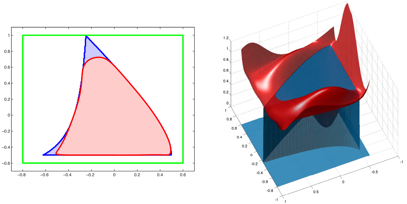
Fig. 4. Left: degree 8 inner PSS approximation (red) of stabilizability region \mathcal{K} (inner surface in light blue). Right: degree 8 polynomial approximation (upper surface in red) of the indicator function (lower surface in blue) of \mathcal{K} .
