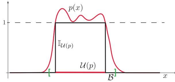
Fig. 1. Illustration of Chebyshev’s inequality: the polynomial is always greater or equal than the indicator function of p(x) \geq 1 , hence the integral of p over \mathcal{B} is always an upper bound of the volume of \mathcal{U}(p) .
