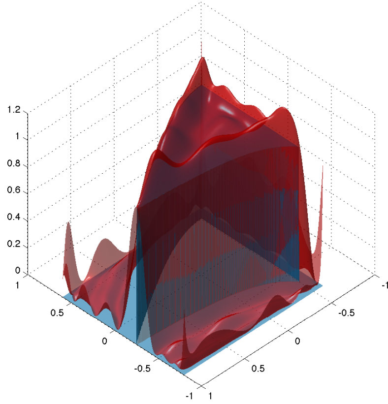
Fig. 3. Degree 20 polynomial approximation (upper surface in red) of the indicator function (lower surface in blue) of the nonconvex planar stabilizability region \mathcal{K} .
