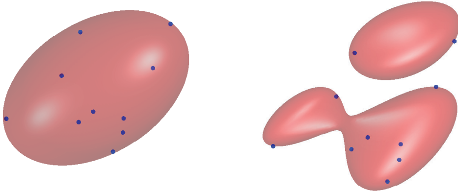
Fig. 7. Including the same 10 space points (blue) in PSS of degree 4 (left) and 10 (right).
