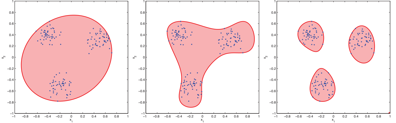
Fig. 6. Minimum L^1 -norm PSS at 100 points (blue), for degree 2 (left), 5 (center), and 9 (right).
