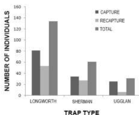
Figure 2.— Numbers of mice captured by trap type as recorded during the present study.
