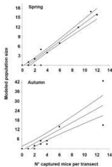
Figure 3.— Relationships (with 95 % confidence intervals) between used simple indices of relative abundance (number of individuals per sampling effort per line) and modelled population sizes. For statistical details, see the text.
