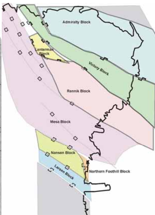
Fig. 2 Sketch map showing the eight rigid crustal blocks dissected out by the active fault network in NVL during the recording time
