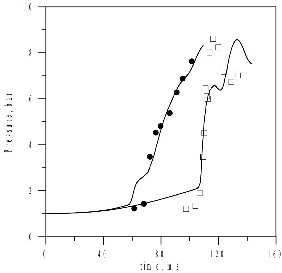
Figure 1 – Validation of the CFD code with experiments: pressure as function of time in linked vessels. 10% methane-air mixture, ( ) simulations, (●) central ignition experiment, (□) end ignition experiment
